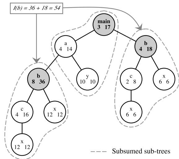
Figure 3: Subsumed subtrees for Example 1
