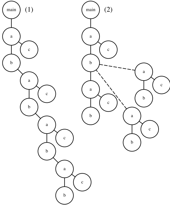
Figure 5: CCT before (1) and after (2) the recursive adjustment
