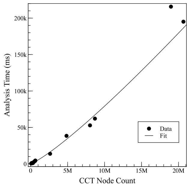
Figure 6: Analysis Time vs CCT Size
