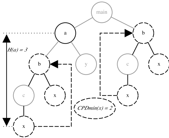
Figure 4: CCT for Example 1 showing height and CPD_{min}
