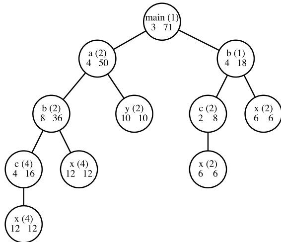
Figure 1: CCT for Example 1
